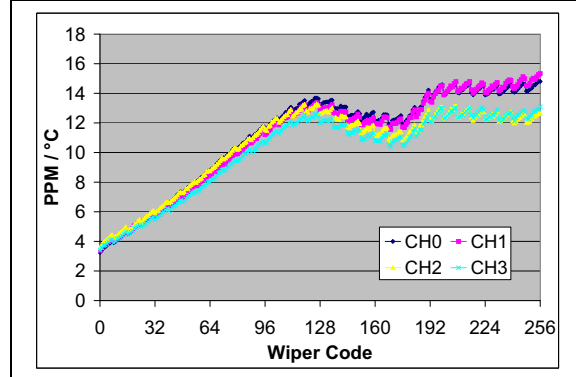
FIGURE 2-62: 100\text{ k}\Omega – R_{WB} PPM/ ^\circ\text{C} vs. Wiper Setting. ( R_{BW}(\text{code}=n, 125^\circ\text{C}) - R_{BW}(\text{code}=n, -40^\circ\text{C}) ) / R_{BW}(\text{code} = 256, 25^\circ\text{C}) / 165^\circ\text{C} * 1,000,000 ) ( V_{DD} = 3.0\text{V} , I_W = 24\text{ }\mu\text{A} ).
