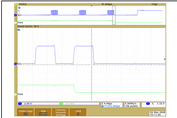
FIGURE 2-48: 50\text{ k}\Omega – Low-Voltage Decrement Wiper Settling Time ( V_{DD} = 2.7\text{V} ) ( 1\text{ }\mu\text{s/Div} ).
