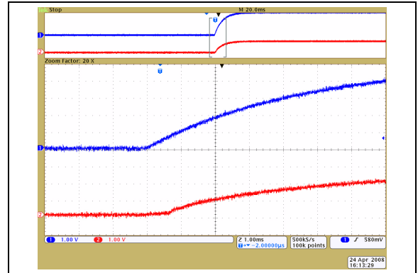
FIGURE 2-50: 50\text{ k}\Omega – Low-Voltage Increment Wiper Settling Time ( V_{DD} = 2.7\text{V} ) ( 1\text{ }\mu\text{s/Div} ).
