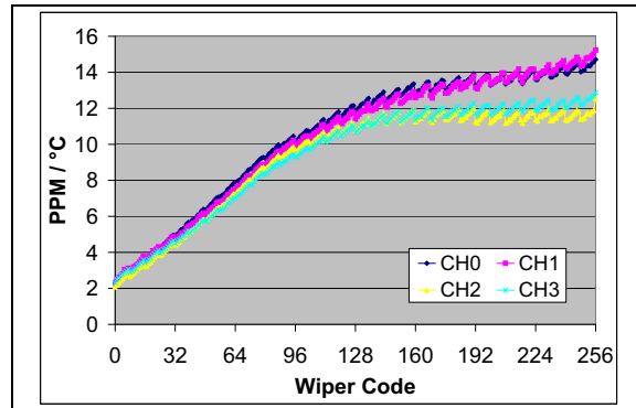
FIGURE 2-61: 100\text{ k}\Omega – R_{WB} PPM/ ^\circ\text{C} vs. Wiper Setting. ( R_{BW}(\text{code}=n, 125^\circ\text{C}) - R_{BW}(\text{code}=n, -40^\circ\text{C}) ) / R_{BW}(\text{code} = 256, 25^\circ\text{C}) / 165^\circ\text{C} * 1,000,000 ) ( V_{DD} = 5.5\text{V} , I_W = 45\text{ }\mu\text{A} ).
