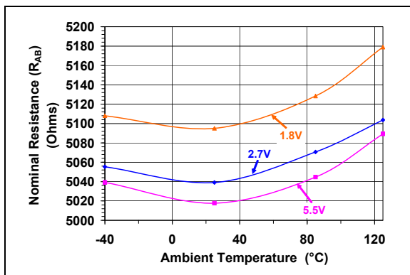
FIGURE 2-11: 5.0 kΩ: Nominal Resistance ( R_{AB} ) vs. Temperature and V_{DD} .
