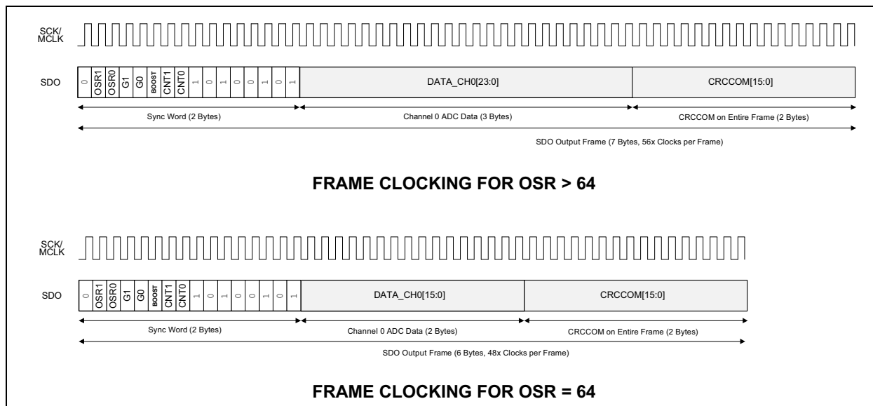
FIGURE 7-2: Frame Word.
