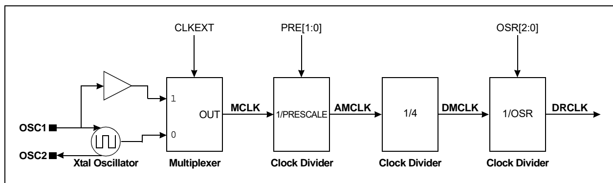
FIGURE 4-1: Clock Sub-Circuitry.
