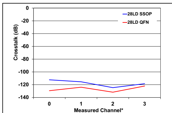
FIGURE 2-32: Crosstalk vs. Measured Channel.
