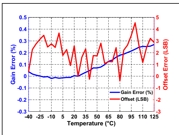
FIGURE 3-37: Gain and Offset Error Drifts Vs. Temperature using Internal Reference, with Respect to 25°C: f_S = 80 Msp/s, f_{IN} = 14.7 MHz, V_{SENSE} = AV_{DD12} , Resolution = 16-bit, A_{IN} = -1 dBFS.
