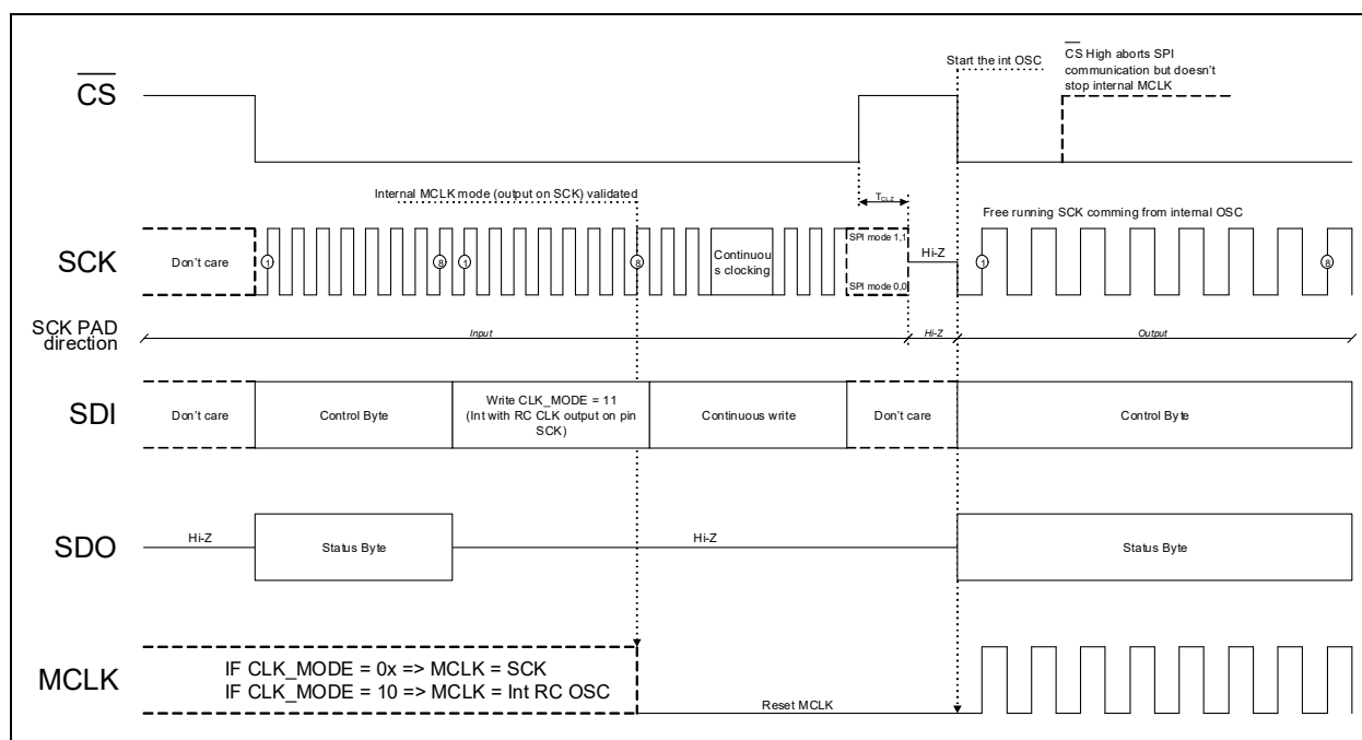
FIGURE 6-15: MCP3565R Transition from CLK_SEL[1:0] = 0x/10 to 11.
