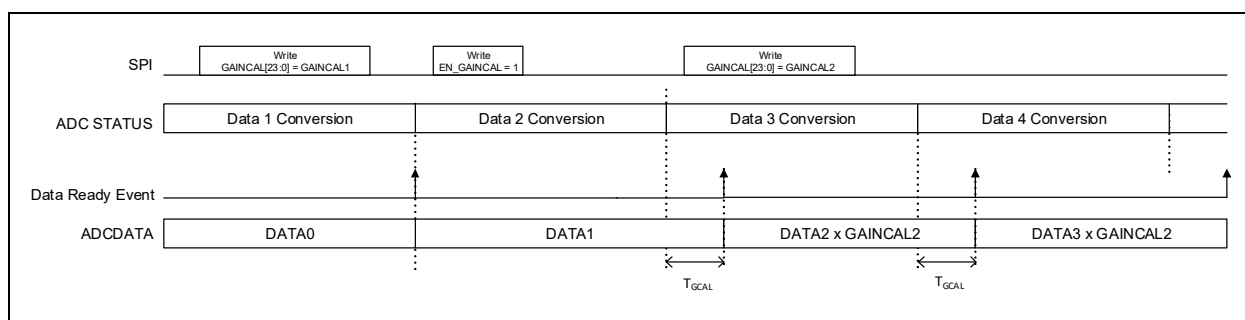
FIGURE 5-13: ADC Output and Data Ready Event Behavior with Digital Gain Error Calibration Enabled.
