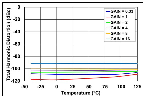
FIGURE 2-28: THD vs. Temperature, External V_{REF} .
