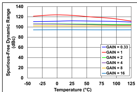
FIGURE 2-29: SFDR vs. Temperature, External V_{REF} .
