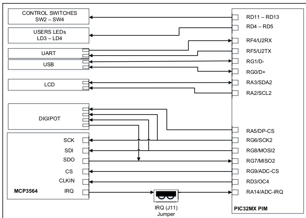
FIGURE 2-3: PIM module Peripheral Usage Overview.
