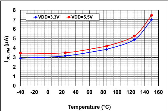
FIGURE 10-2: Average IDDLPM vs. Temperature.
