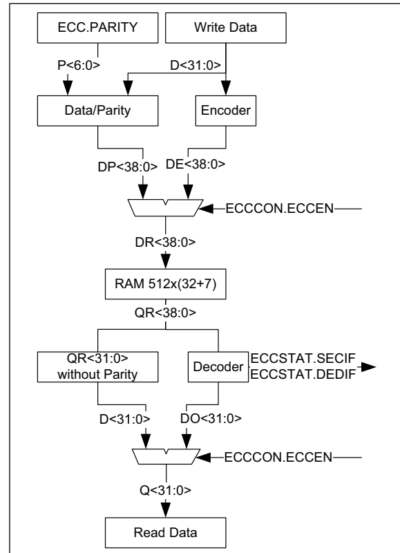
FIGURE 4-3: ECC LOGIC
