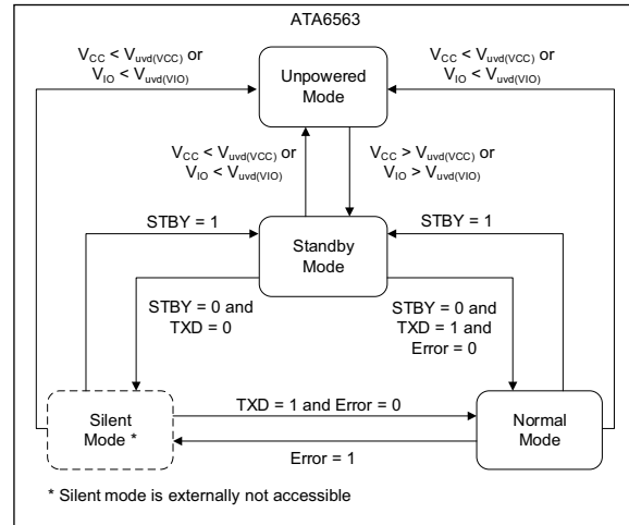
FIGURE 8-1: OPERATING MODES
