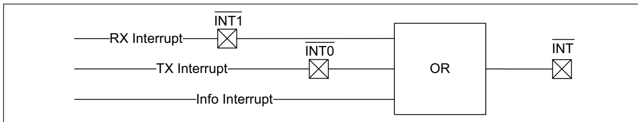
FIGURE 7-1: INTERRUPT PINS
