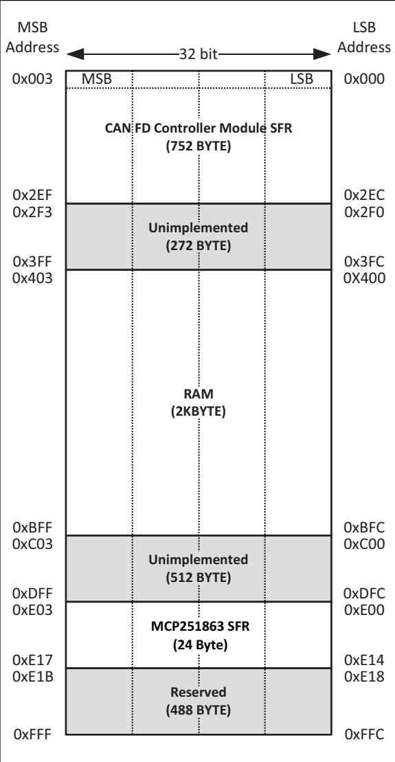
FIGURE 4-1: MEMORY MAP
