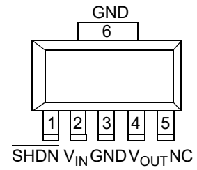
5-Pin SOT-223
