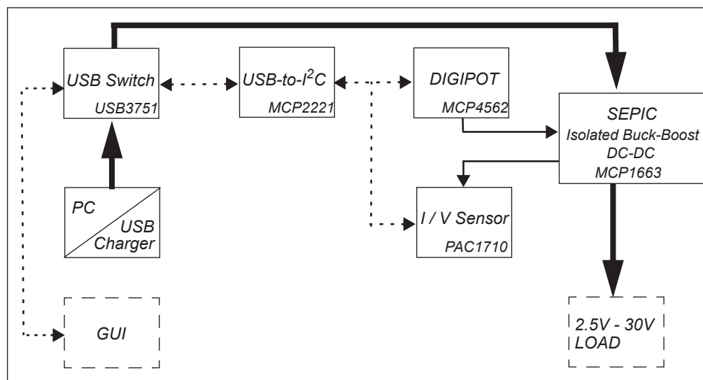
FIGURE 2-1: MCP1663 USB Programmable Power Supply Functional Blocks.
