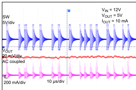
FIGURE 2-25: Light Load Switching Waveforms – MCP16362.
