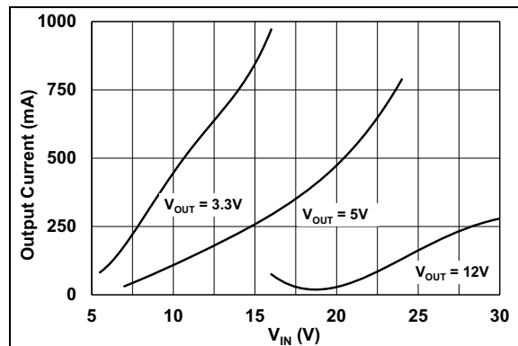
FIGURE 2-18: PFM/PWM Threshold.
