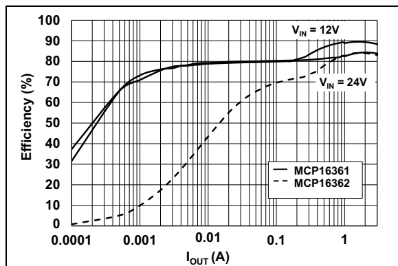
FIGURE 2-2: 5V V_{OUT} Efficiency vs. I_{OUT} .
