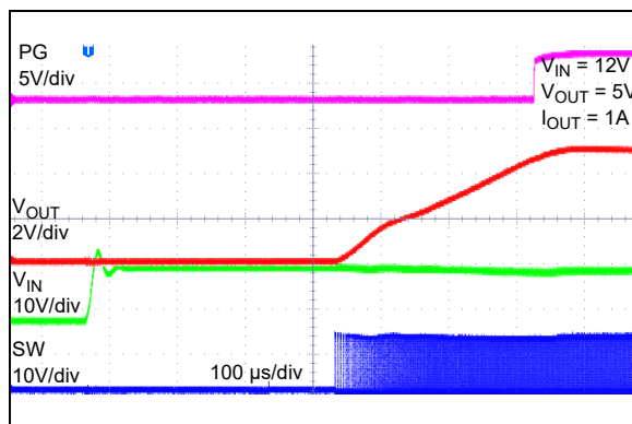
FIGURE 2-27: Start-Up from V_{IN} .
