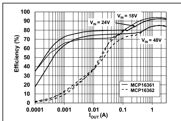
FIGURE 2-3: 12V V_{OUT} Efficiency vs. I_{OUT} .
