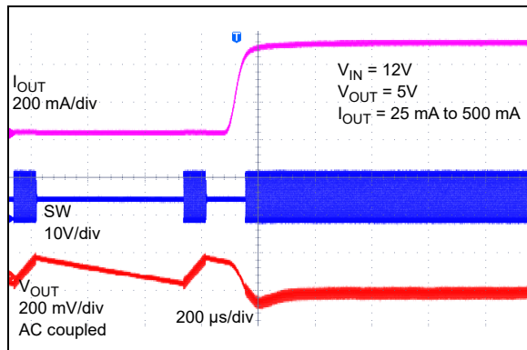
FIGURE 2-26: PFM to PWM Transition.
