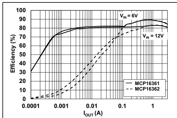
FIGURE 2-1: 3.3V V_{OUT} Efficiency vs. I_{OUT} .
