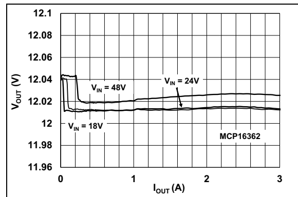
FIGURE 2-6: 12V V_{OUT} vs. I_{OUT} .
