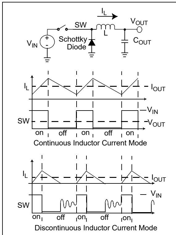
FIGURE 5-1: Step-Down Converter.
