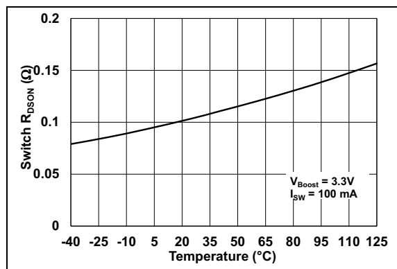
FIGURE 2-10: Switch R_{\text{DS(on)}} vs. Temperature.
