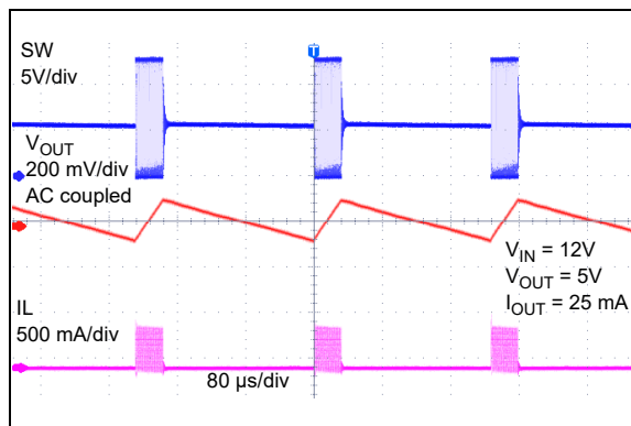
FIGURE 2-24: Light Load Switching Waveforms – MCP16361.
