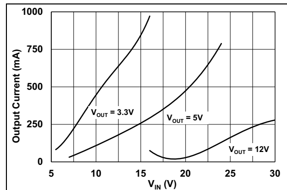
FIGURE 2-18: PFM/PWM Threshold.
