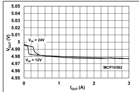
FIGURE 2-5: 5V V_{OUT} vs. I_{OUT} .
