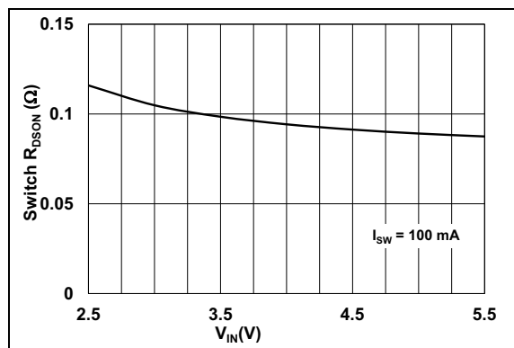
FIGURE 2-11: Switch R_{\text{DS(on)}} vs. V_{\text{BOOST}} .
