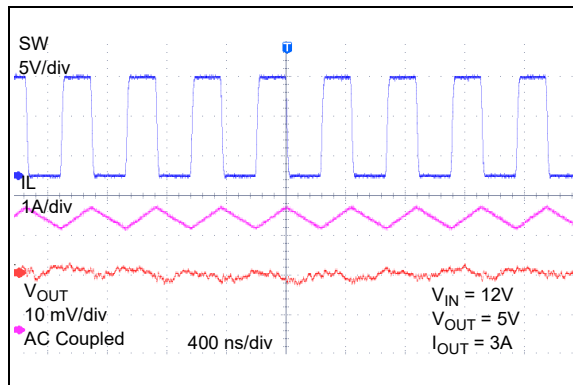
FIGURE 2-23: Heavy Load Switching Waveforms.
