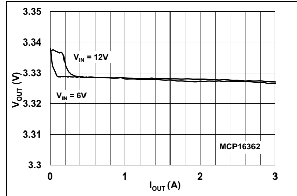
FIGURE 2-4: 3.3V V_{OUT} vs. I_{OUT} .
