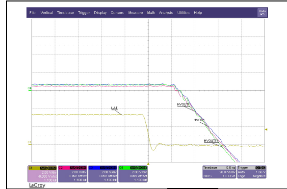
FIGURE 1-17: Typical LATCHB to HV_{OUT} Propagation Delay
