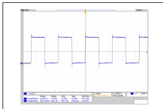
FIGURE 1-23: Typical VSSPUL output waveform I_o = -5mA .
