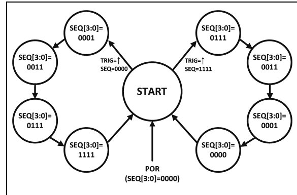
FIGURE 3-8: Sequence On/Off Control State Diagram.
