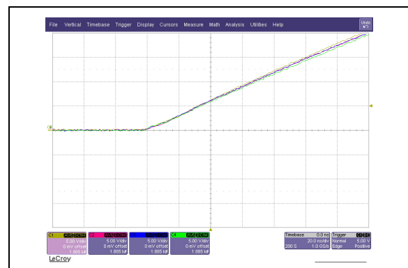
FIGURE 1-15: Typical HV OUT Channel-to-Channel Delay
