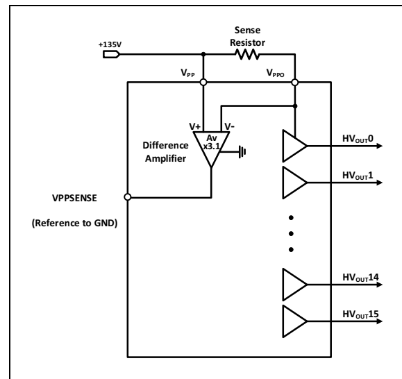
FIGURE 3-11: Current Sensing Topology.
