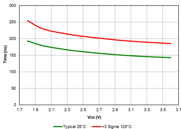
Figure 41-85. Comparator Response Time Falling Edge, PIC16F18426/46 only
