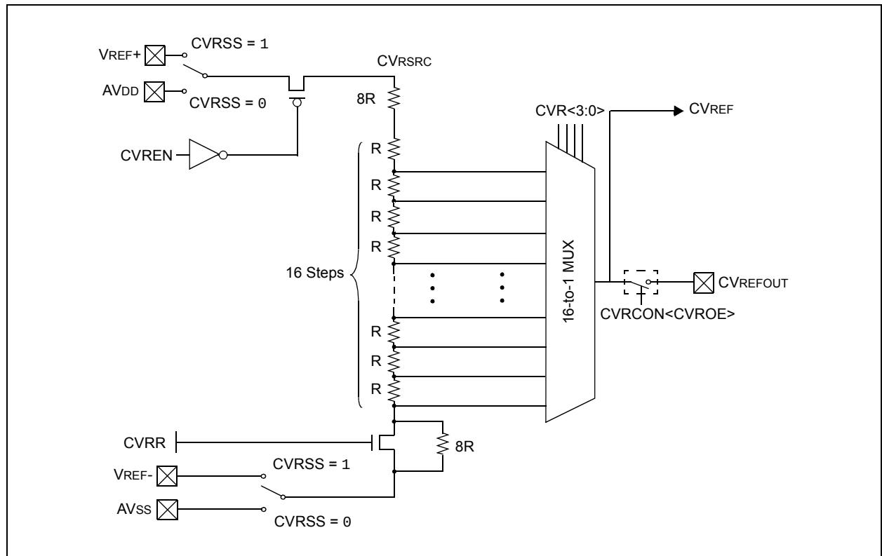
FIGURE 33-1: COMPARATOR VOLTAGE REFERENCE BLOCK DIAGRAM
