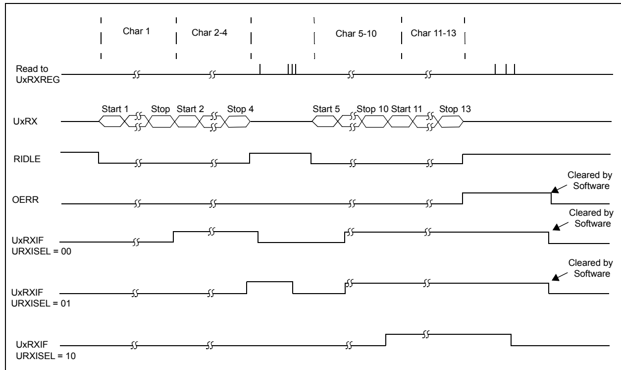
FIGURE 24-2: UART RECEPTION
