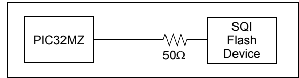
FIGURE 2-8: SERIES RESISTOR
