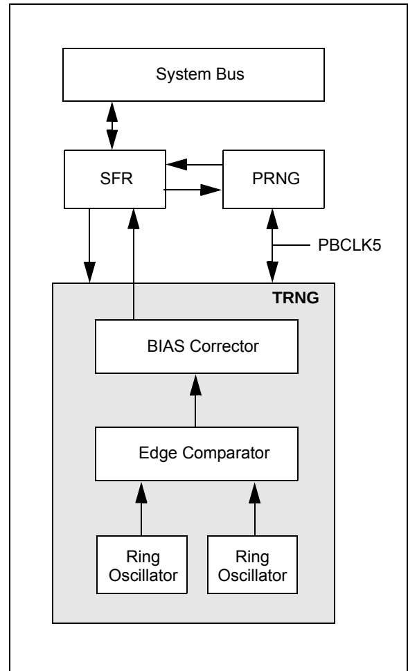
FIGURE 28-1: RANDOM NUMBER GENERATOR BLOCK DIAGRAM
