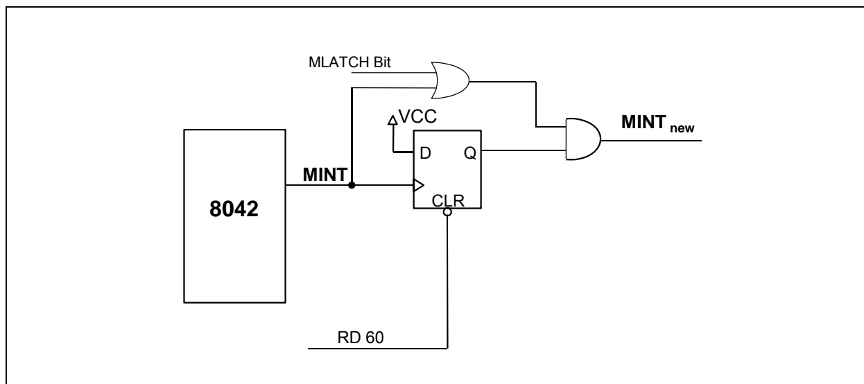
FIGURE 6-5: MOUSE LATCH
