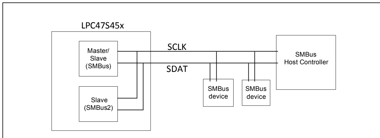
FIGURE 6-10: REPRESENTATIVE DIAGRAM OF SMBUS AND SMBUS2
