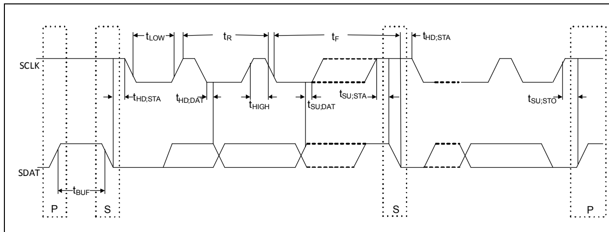
FIGURE 11-24: SMBUS TIMING
