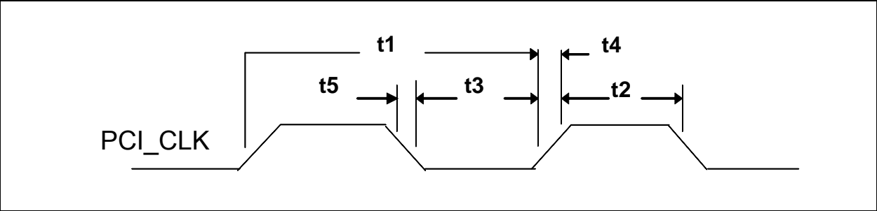
FIGURE 11-3: PCI CLOCK TIMING
