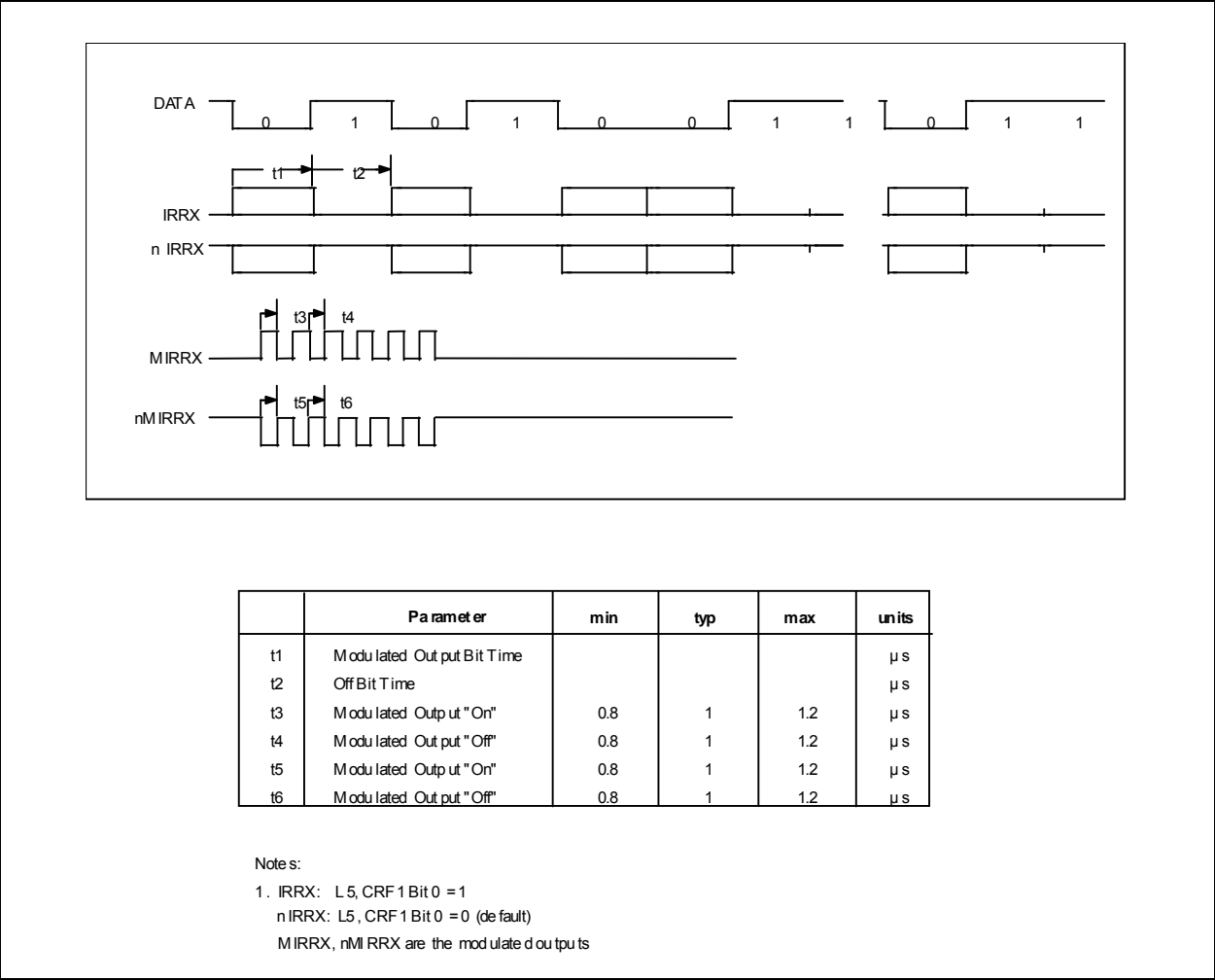
FIGURE 11-22: AMPLITUDE SHIFT KEYED IR RECEIVE TIMING
