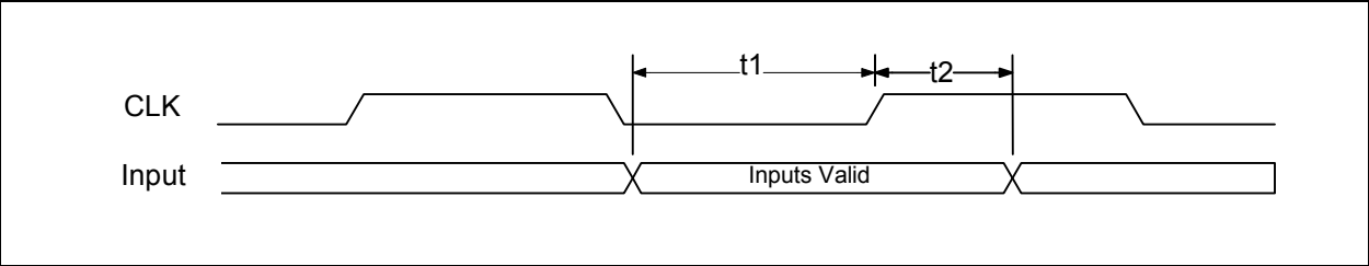
FIGURE 11-6: INPUT TIMING MEASUREMENT CONDITIONS, LPC SIGNALS
