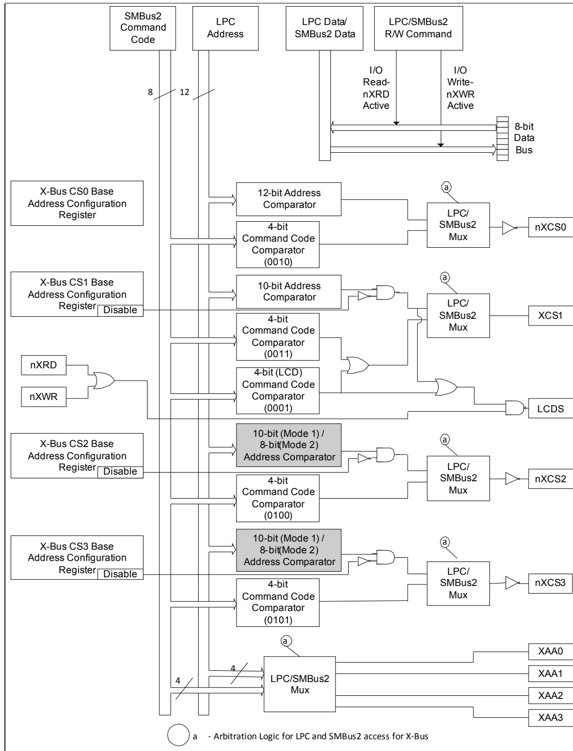
FIGURE 6-13: LPC AND SMBUS I/O ACCESSSES TO THE X-BUS INTERFACE (MODE 1/MODE 2)
