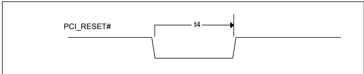
FIGURE 11-4: RESET TIMING
