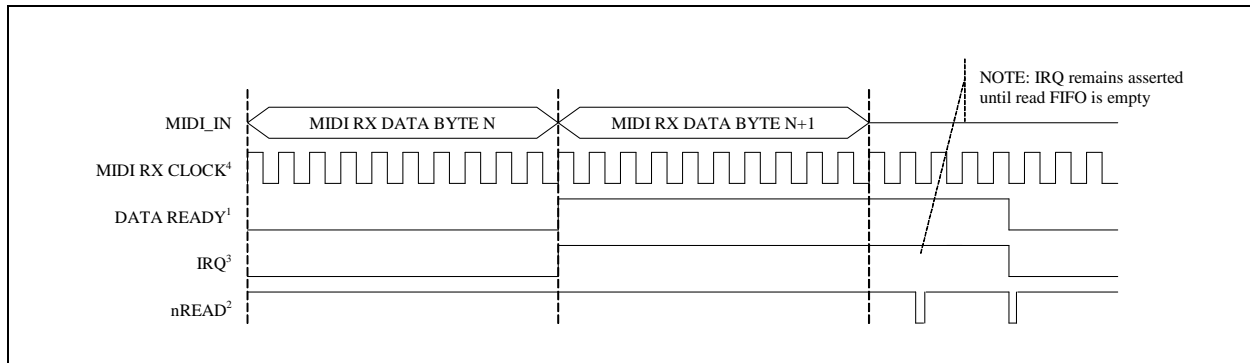
FIGURE 9-2: MPU-401 INTERRUPT
