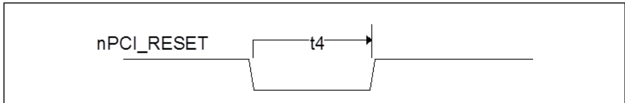
FIGURE 22-4: RESET TIMING
