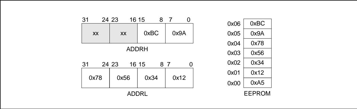
FIGURE 5-2: Example ADDRH, ADDRH and EEPROM Setup
