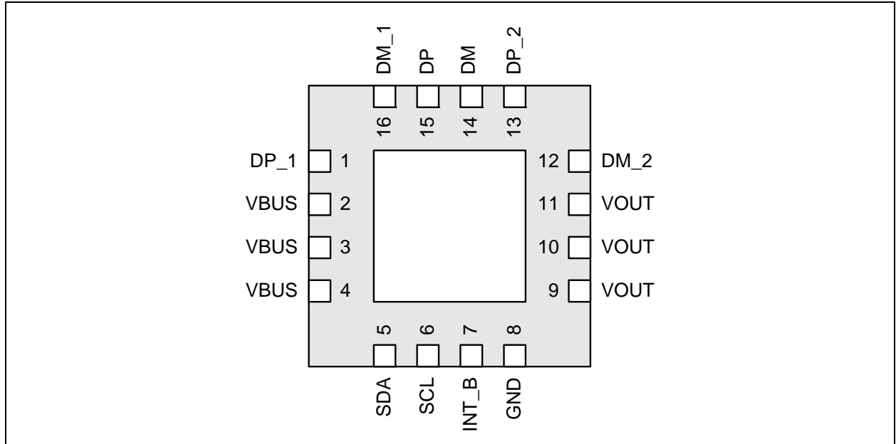
FIGURE 2-2: QFN PACKAGE DIAGRAM (USB3751)
