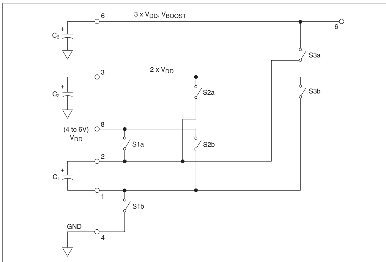
FIGURE 3-3: Voltage Booster.
