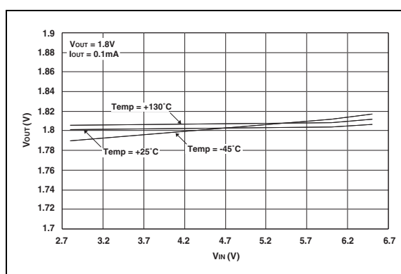
FIGURE 2-12: Dropout Voltage vs. Supply Voltage.
