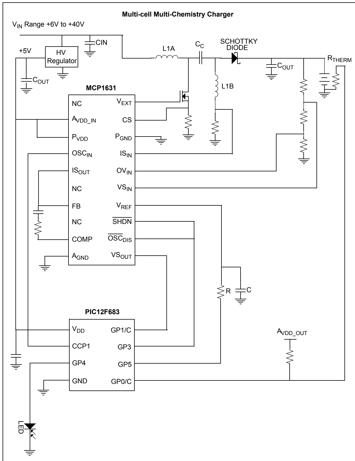
FIGURE 5-3: Wide Range High Voltage Input.
