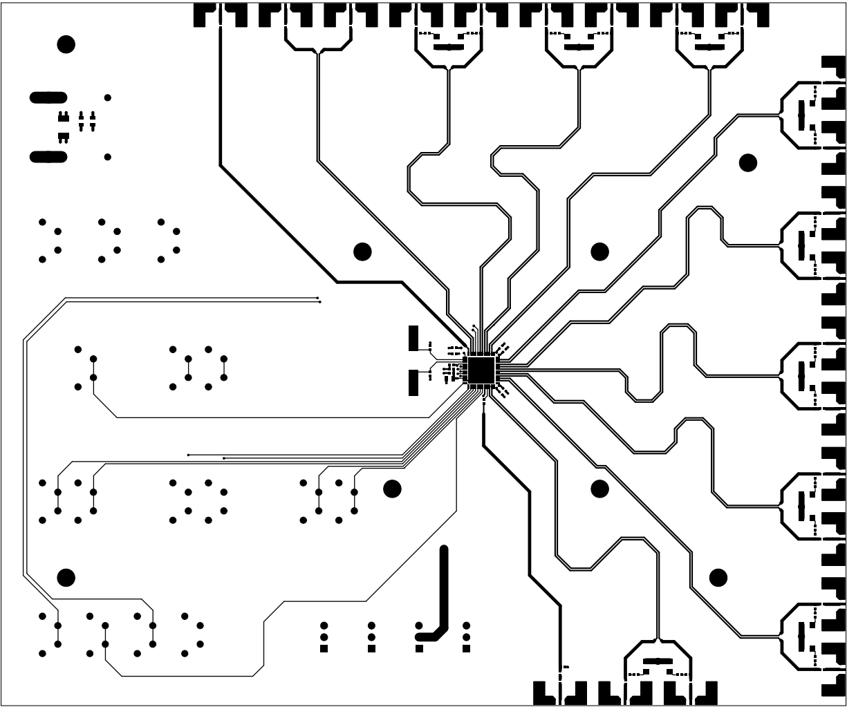
Figure 4. MAX3637 EV Kit PCB Layout—Component Side
