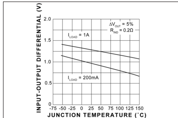
FIGURE 2-11: Dropout Voltage.
