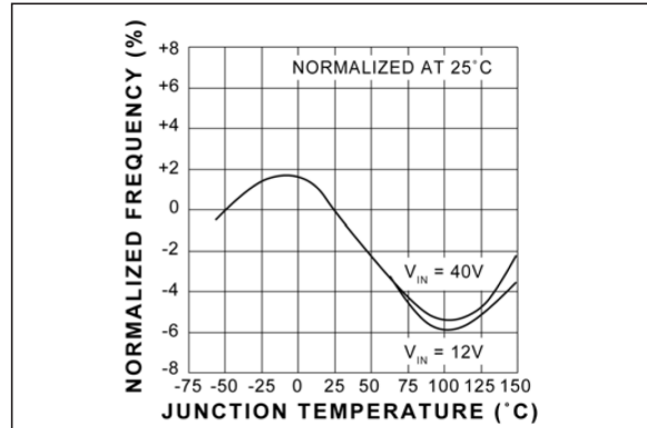
FIGURE 2-10: Oscillator Frequency.
