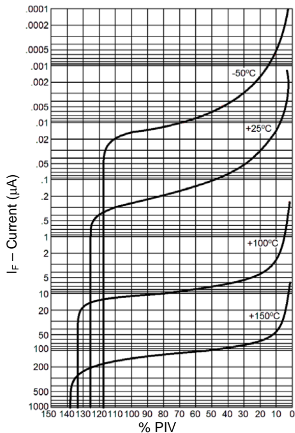
FIGURE 1 Typical Reverse Current vs. PIV
