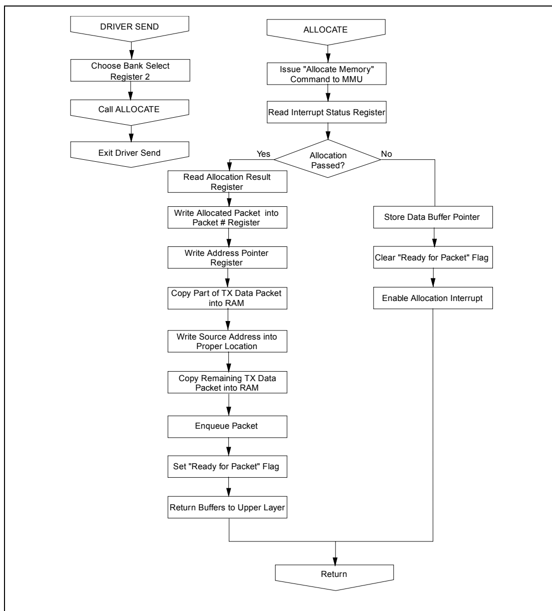
Figure 8.5 – Driver Send and Allocate Routines
