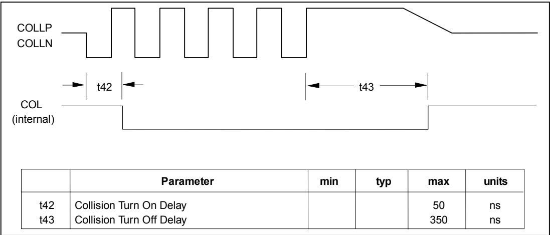
Figure 12.14 – Collision and Timing (AUI)
