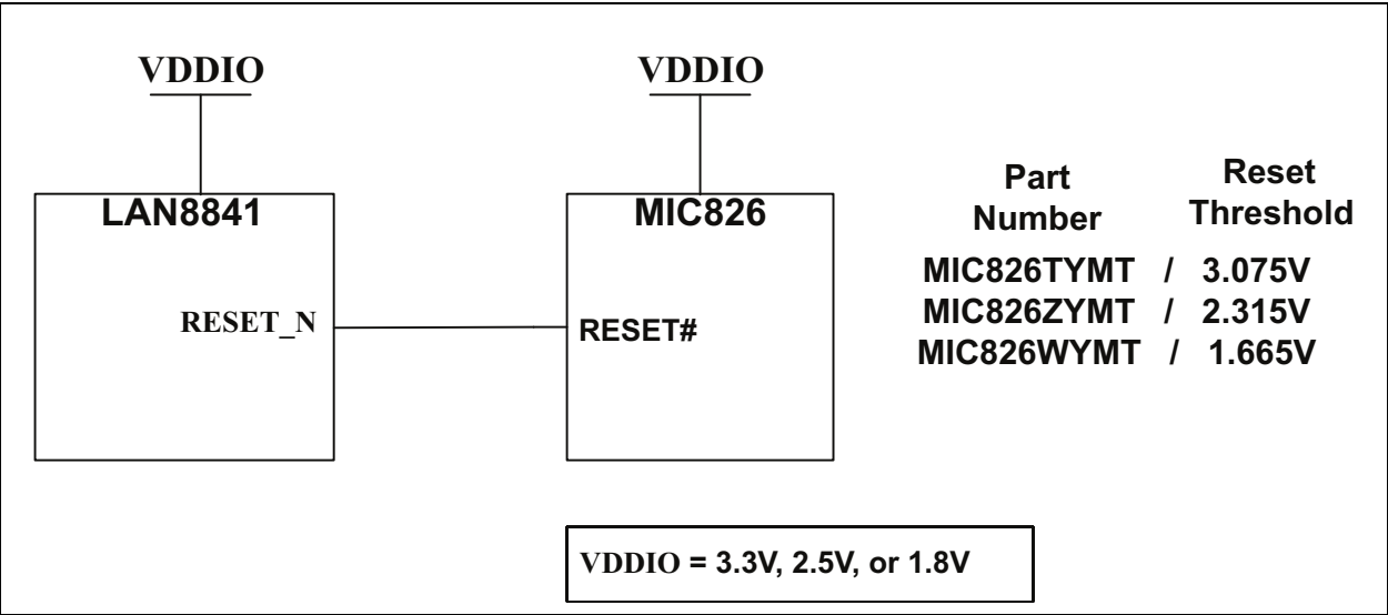
FIGURE 6-19: RESET CIRCUIT WITH MIC826 VOLTAGE SUPERVISOR
