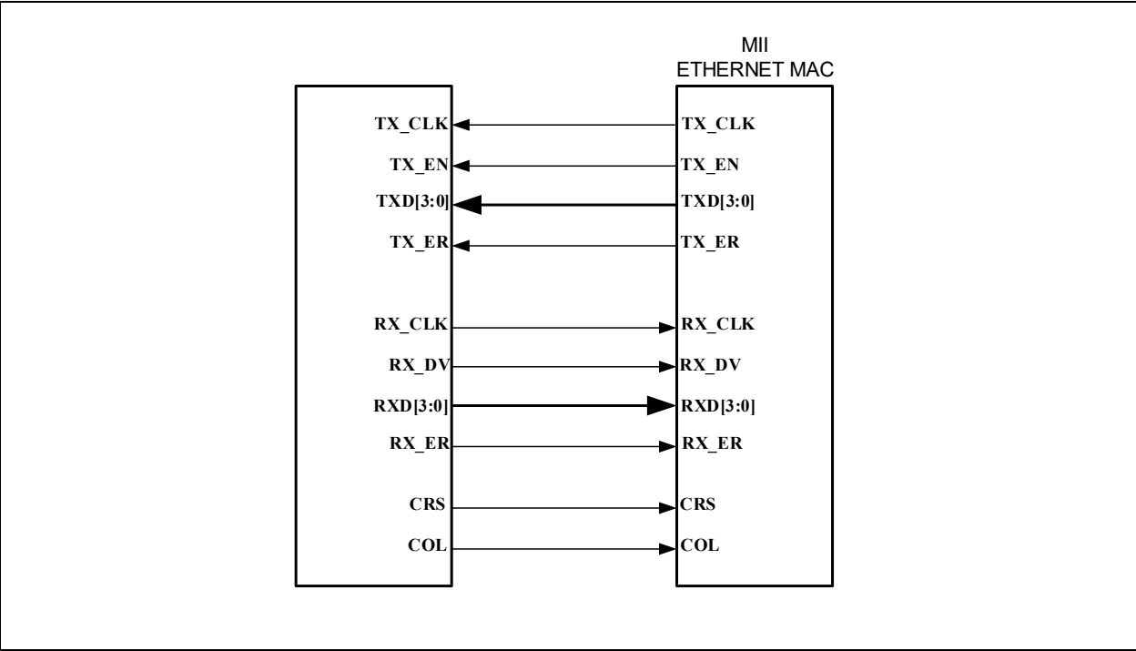
FIGURE 5-17: MII INTERFACE
