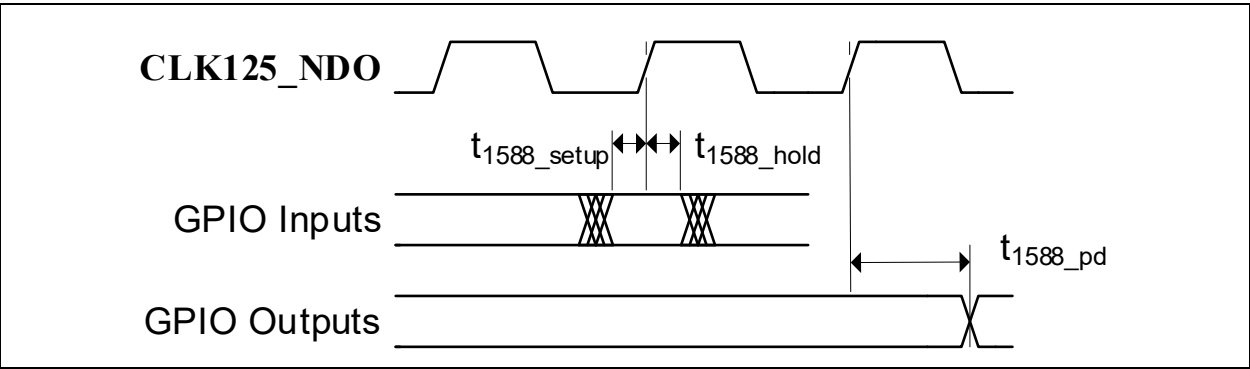
FIGURE 6-16: 1588 GPIO SYNCHRONOUS INPUT TIMING
