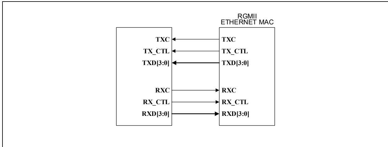
FIGURE 5-18: RGMII INTERFACE
