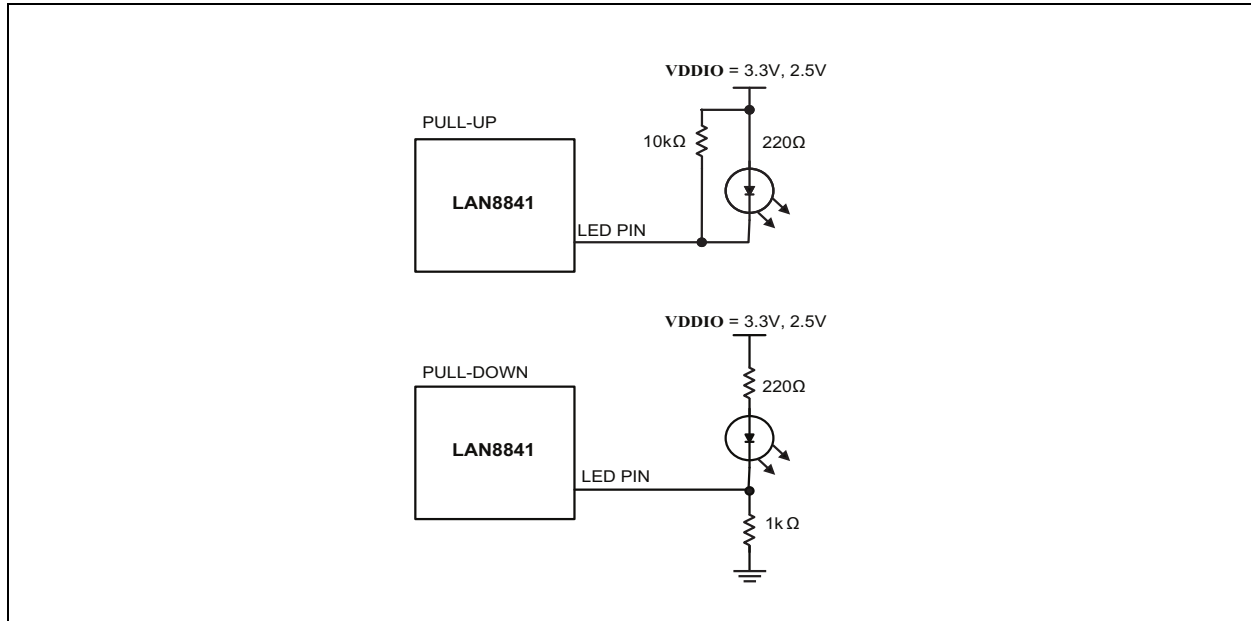
FIGURE 6-20: REFERENCE CIRCUITS FOR LED STRAPPING PINS
