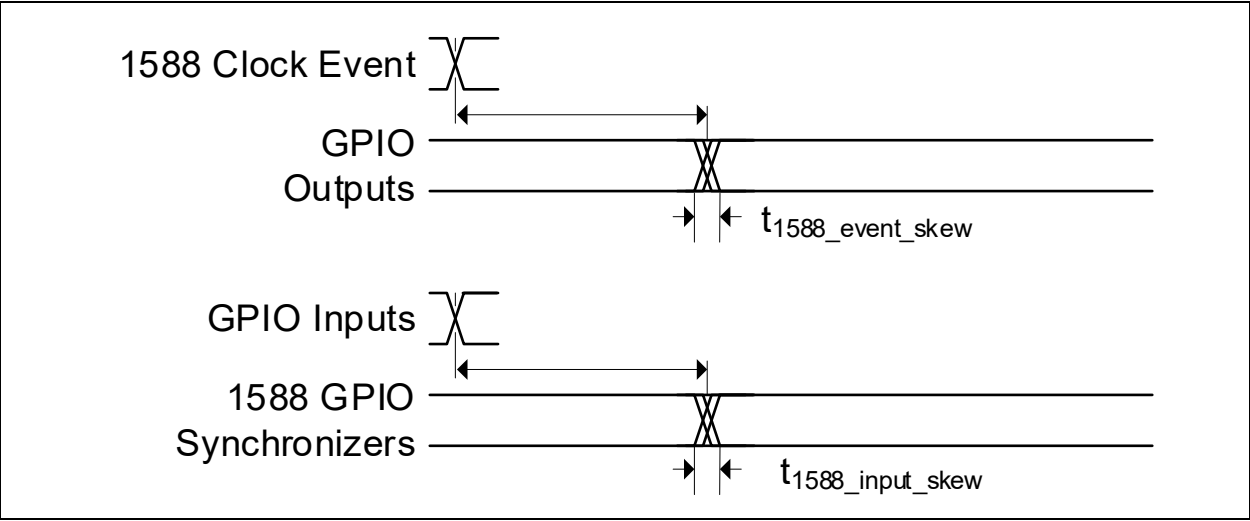
FIGURE 6-15: 1588 GPIO ASYNCHRONOUS INPUT AND OUTPUT TIMING
