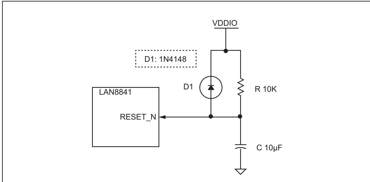
FIGURE 6-17: RESET CIRCUIT IF TRIGGERED BY THE POWER SUPPLY
