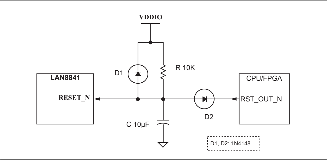
FIGURE 6-18: RECOMMENDED RESET CIRCUIT FOR CPU/FPGA RESET OUTPUT
