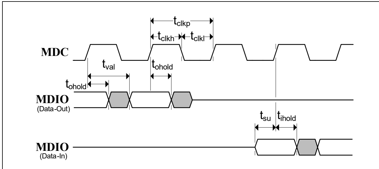
FIGURE 6-9: MDC/MDIO TIMING
