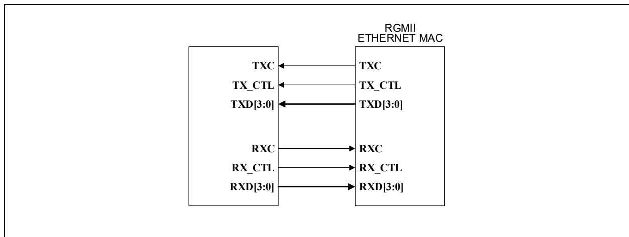
FIGURE 5-12: RGMII INTERFACE
