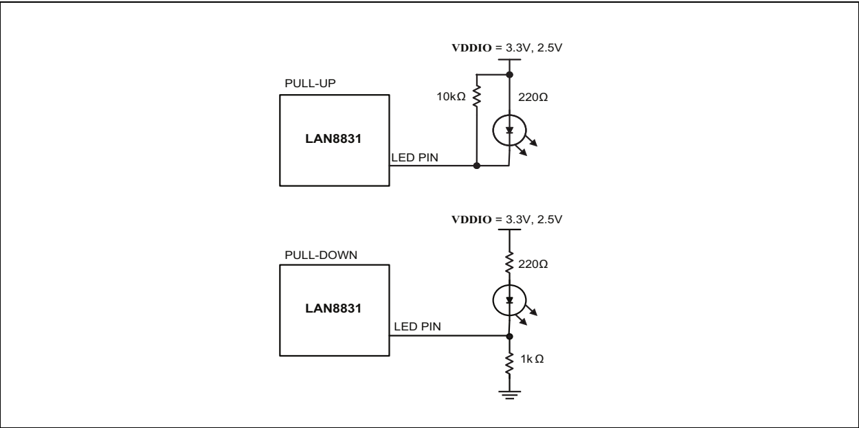
FIGURE 6-17: REFERENCE CIRCUITS FOR LED STRAPPING PINS
