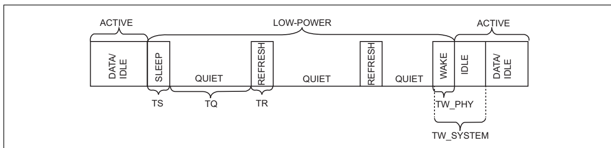
FIGURE 5-8: LPI MODE (REFRESH TRANSMISSIONS AND QUIET PERIODS)
