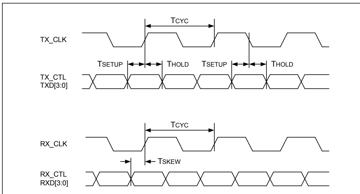
FIGURE 6-1: RGMII TIMING
