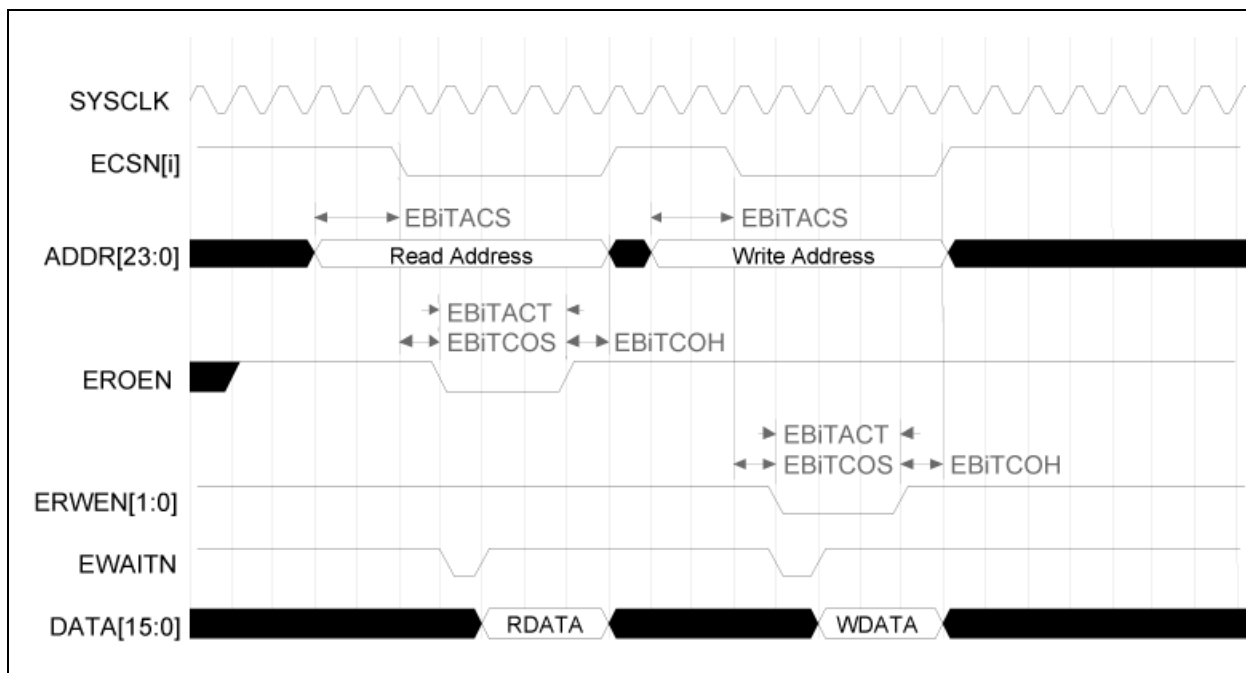
FIGURE 5-4: EXTERNAL I/O READ AND WRITE CYCLES
