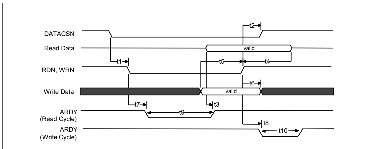
FIGURE 7-3: ASYNCHRONOUS CYCLE – USING DATACSN
