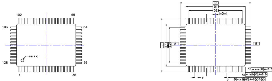
TOP VIEW
