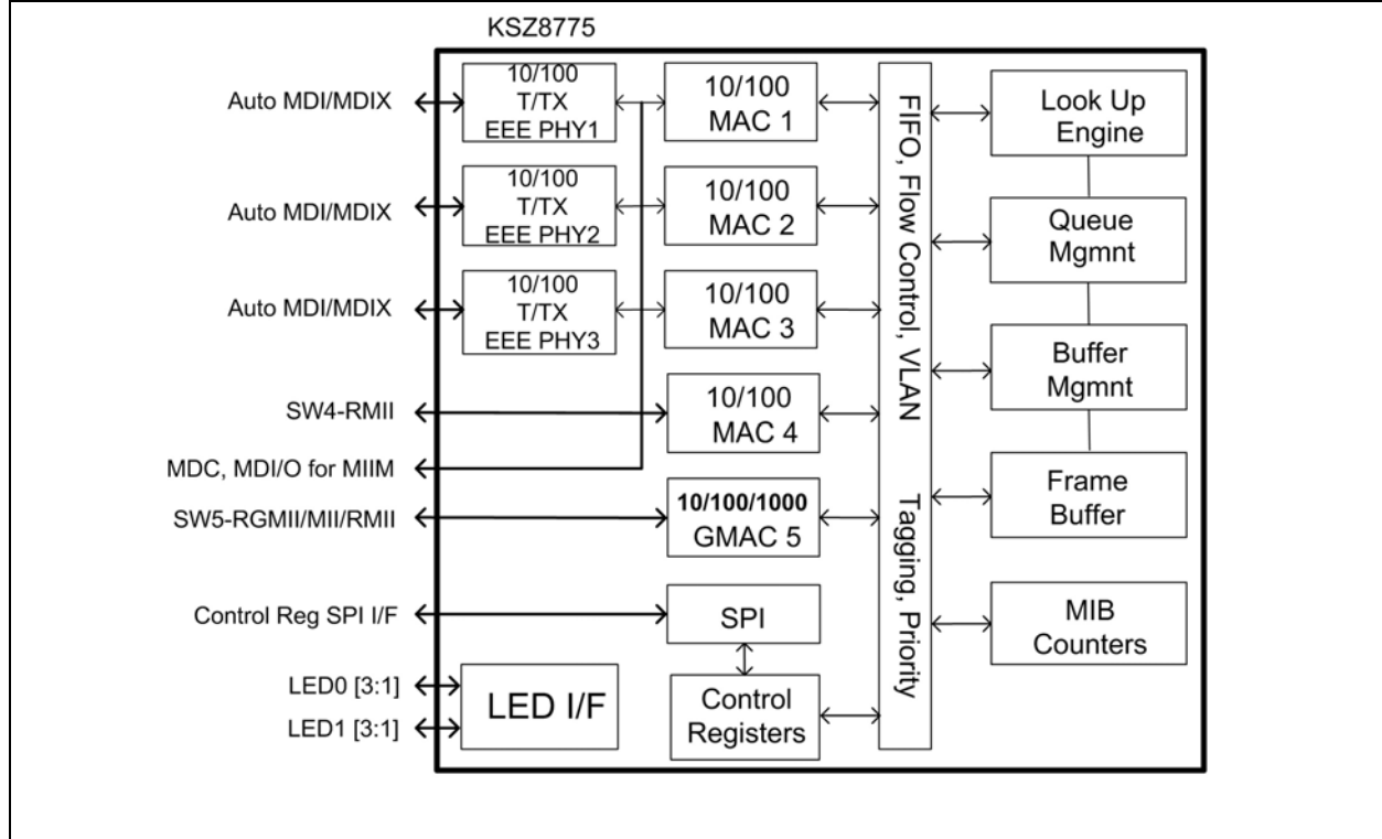
FIGURE 1-1: BLOCK DIAGRAM
