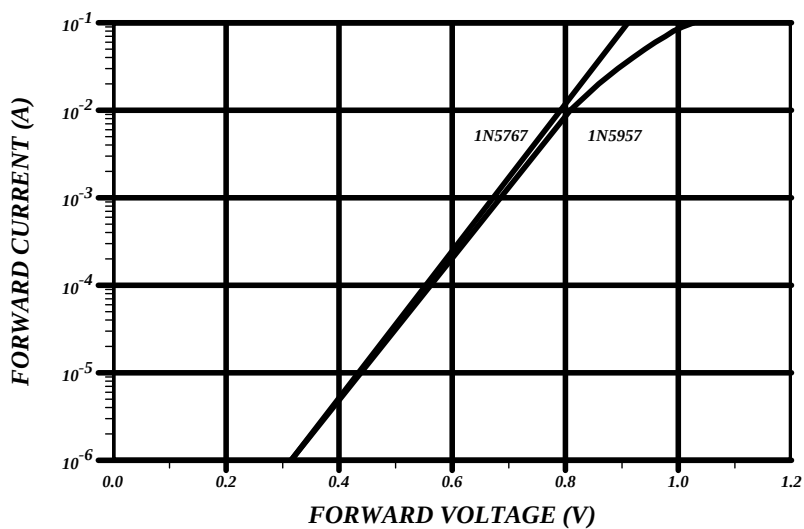
FORWARD VOLTAGE versus CURRENT
