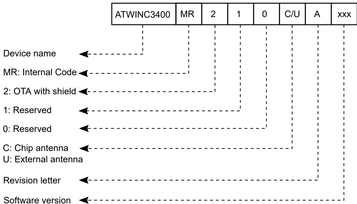
Figure 1-1. Marking Information
