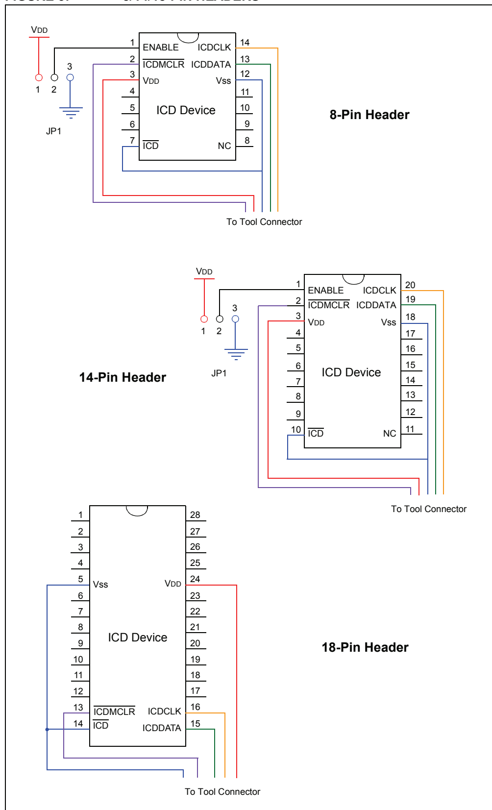
FIGURE 3: 8/14/18-PIN HEADERS
