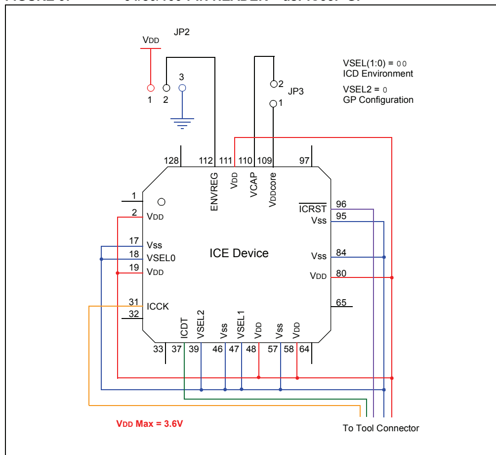
FIGURE 9: 64/80/100-PIN HEADER – dsPIC33F GP
