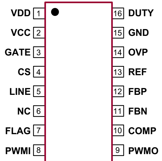
16-Lead SOIC (NG) (top view)
