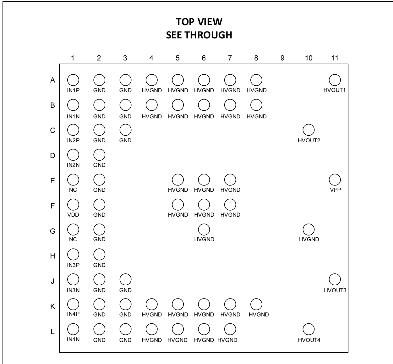
FIGURE 3-2: TFBGA Pinout.
