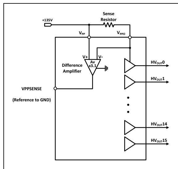
FIGURE 3-4: Current Sensing Topology.
