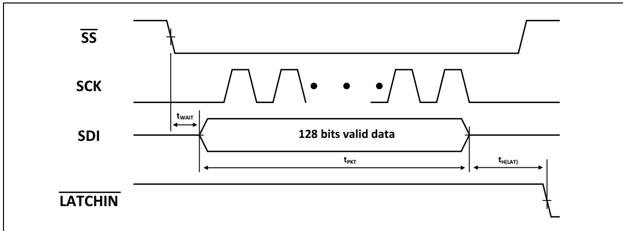
FIGURE 1-1: SPI and LATCHIN Timing Diagram.
