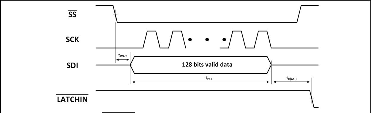
FIGURE 1-1: SPI and LATCHIN Timing Diagram
