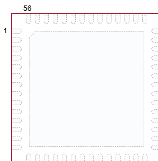
56-lead VQFN (Top view)
