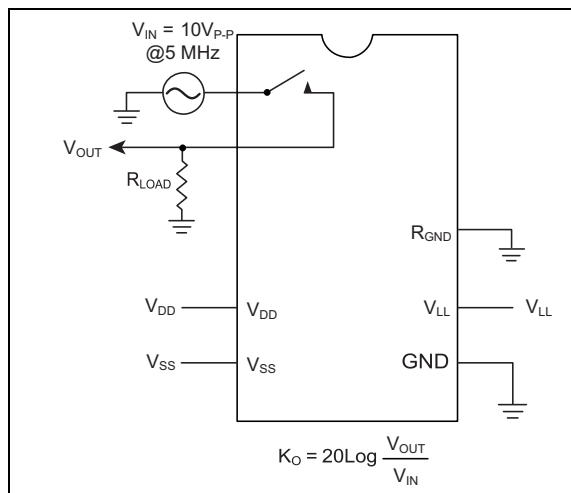
FIGURE 3-6: Off Isolation.
