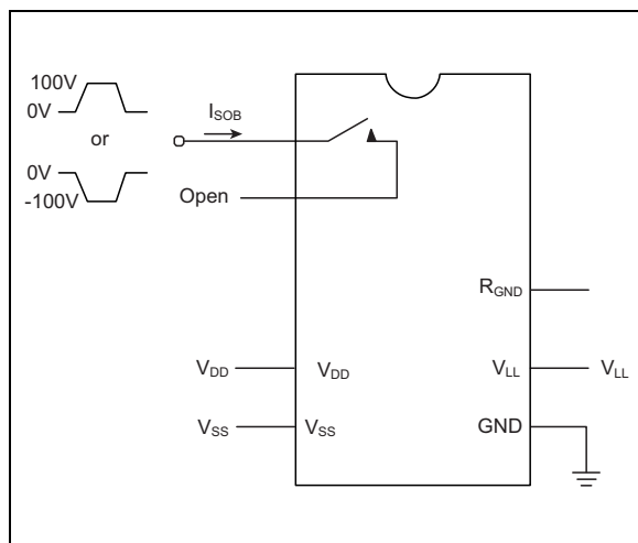
FIGURE 3-2: Switch-Off Bias per Switch.
