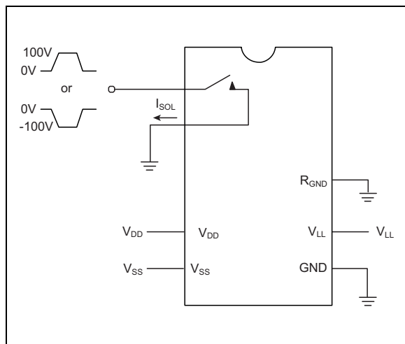
FIGURE 3-1: Switch-Off Leakage per Switch.
