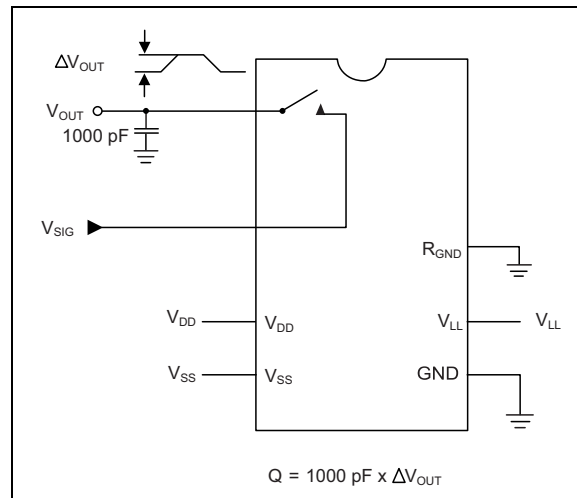
FIGURE 3-9: Charge Injection.
