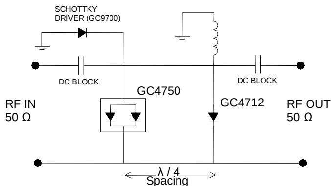
2 Stage Limiter with Schottky Driver
