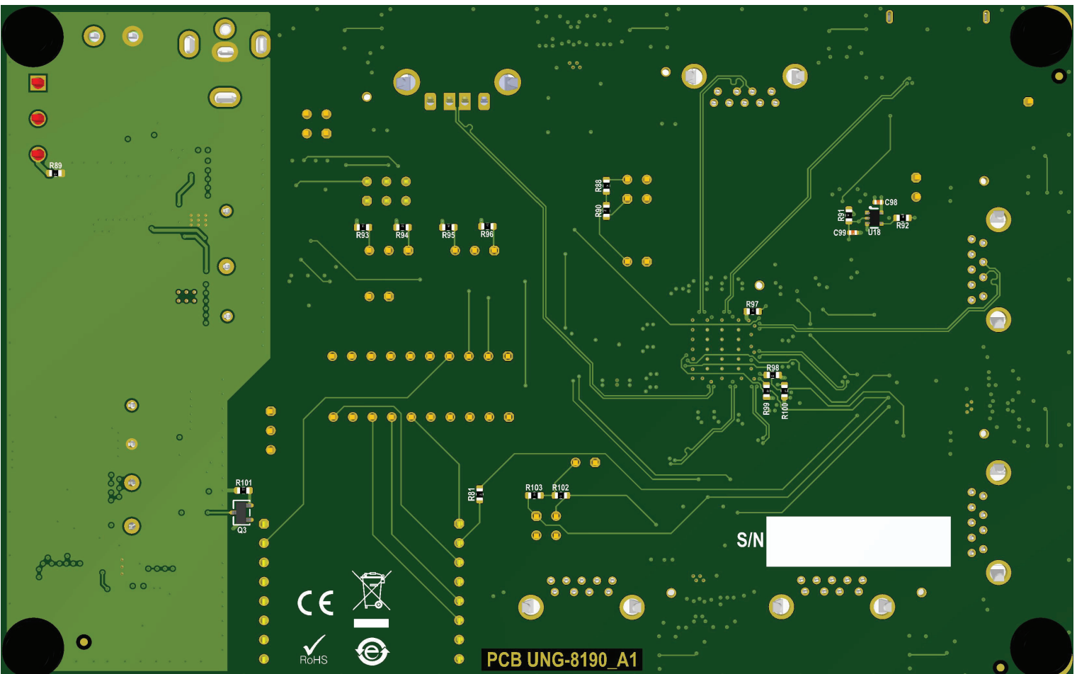
FIGURE C-2: EVB-USB7206 BOTTOM SILK SCREEN IMAGE
