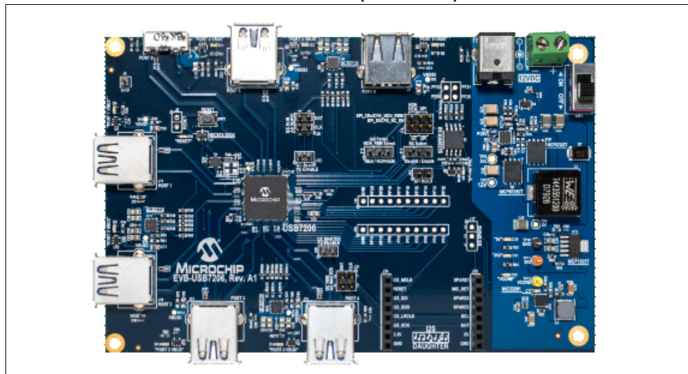
FIGURE 3-1: EVB-USB7206 REV B (TOP VIEW)
