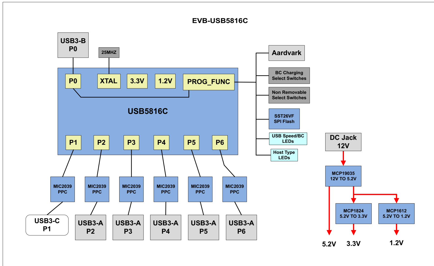
FIGURE 1-1: BLOCK DIAGRAM
