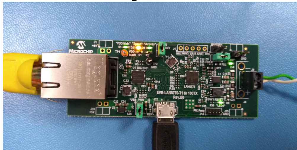
FIGURE 2-1: EVB-LAN8770M_MC EVALUATION BOARD CONNECTIONS
