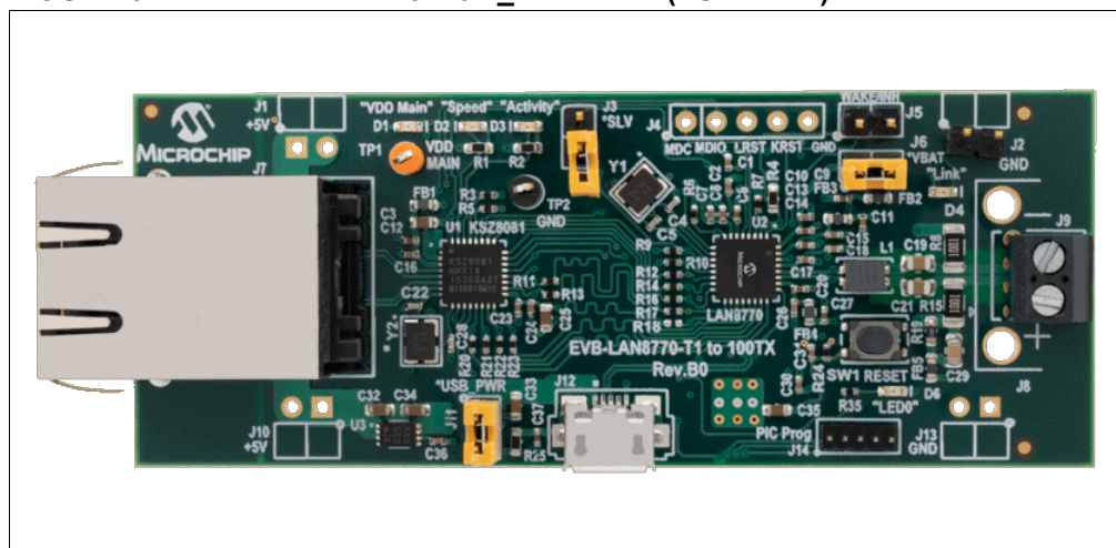
FIGURE 3-1: EVB-LAN8770M_MC REV B (TOP VIEW)
