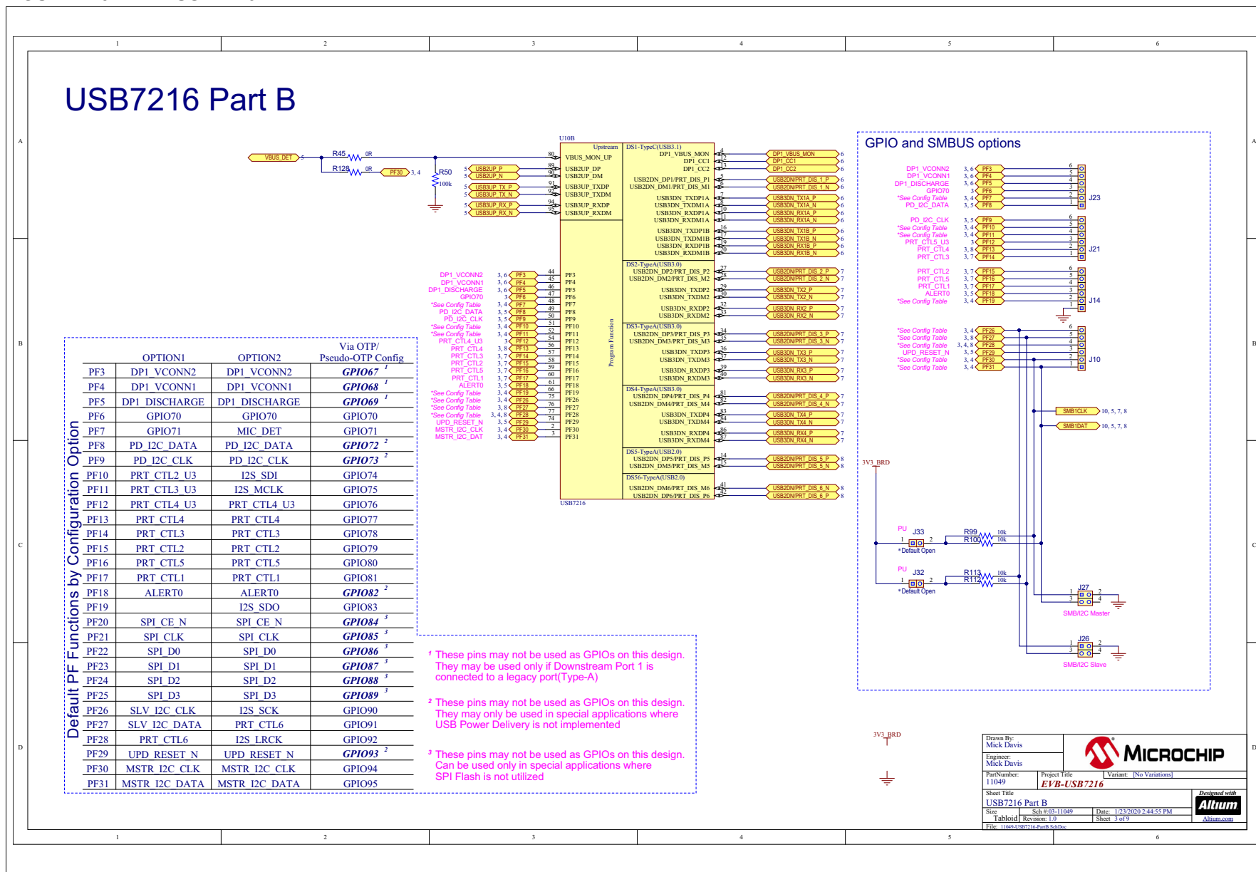
FIGURE A-3: USB7216 PART B
