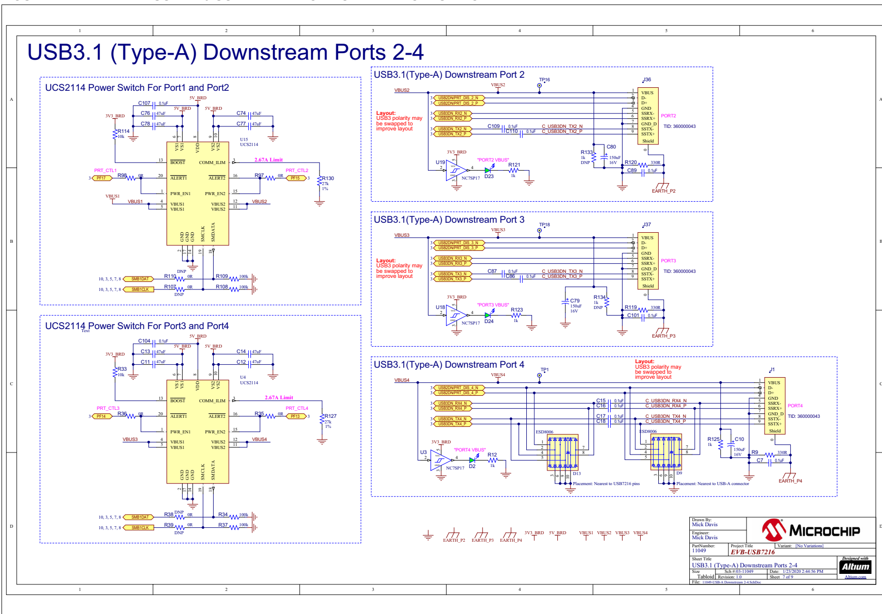
FIGURE A-7: EVB-USB7216 USB TYPE-A DOWNSTREAM PORTS 2 TO 4
